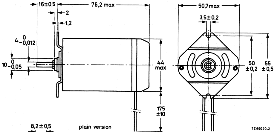
Fig. 1a Version with \phi 4 mm spindle.
