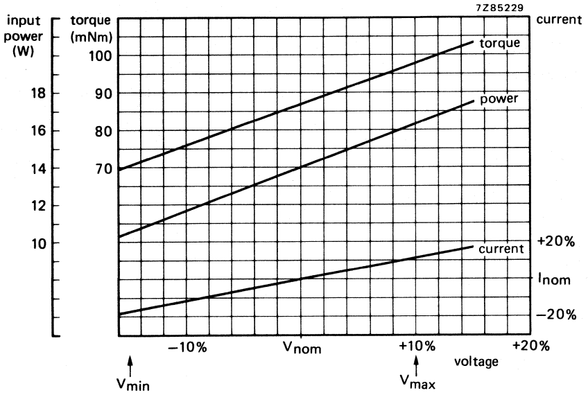
Fig. 3 Typical curves.
