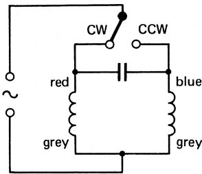
coils in parallel 7Z82271
