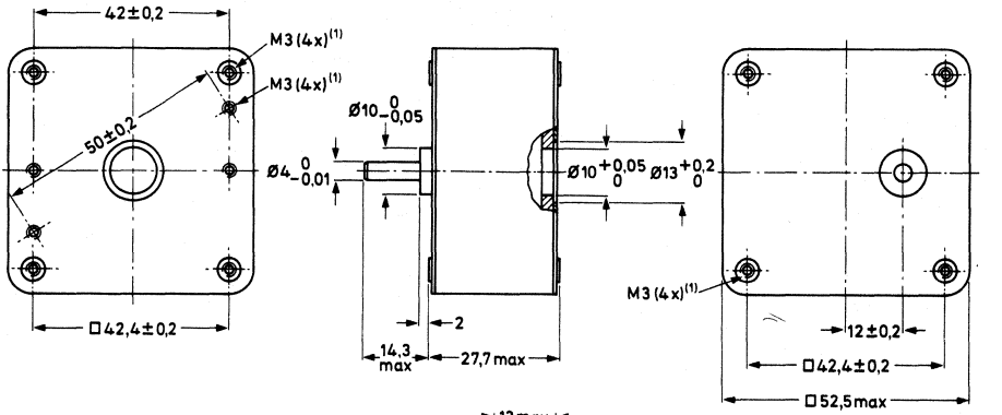
Fig. 2 Type G1, catalogue number 9912 200 01. . .
