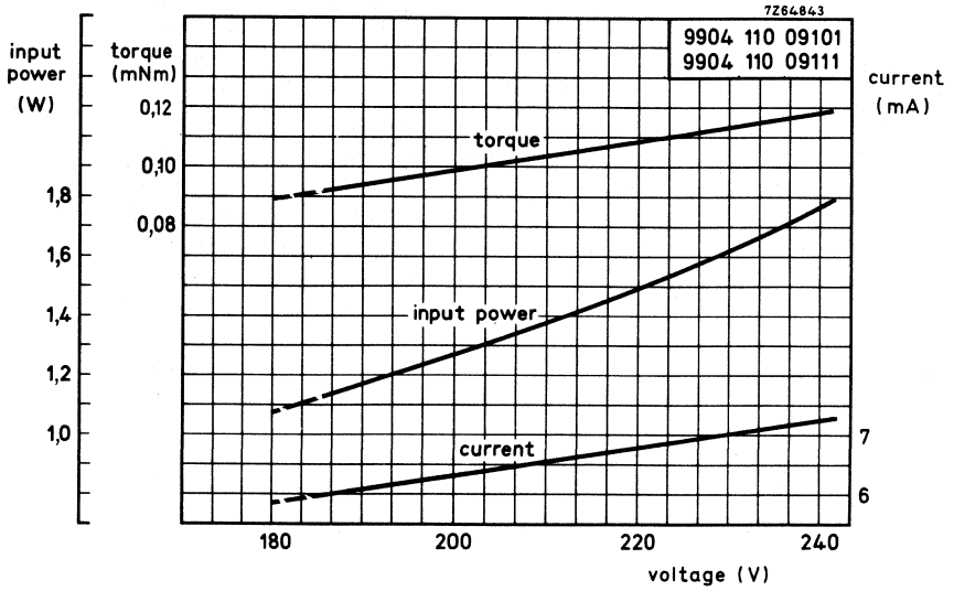
Fig. 4c Typical curves of motors used with a series resistor of 24 kΩ.
