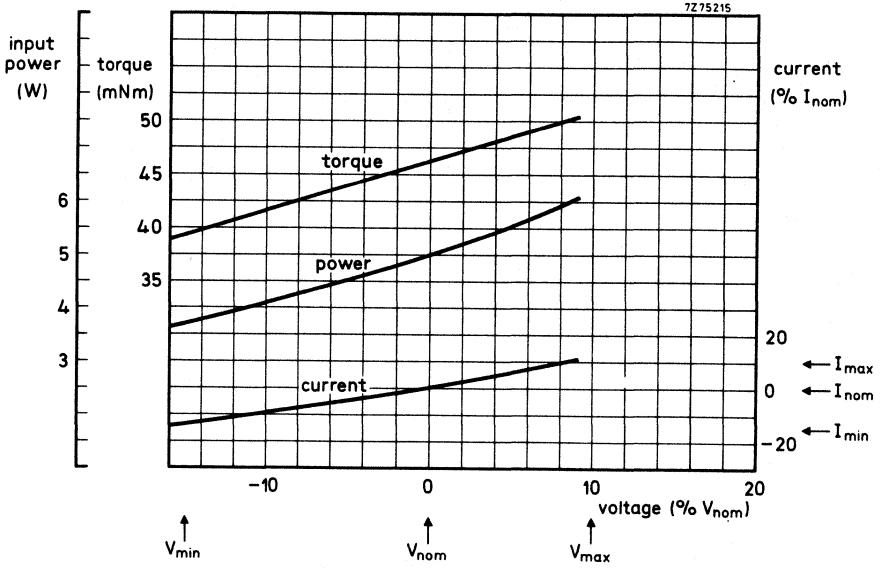
Fig. 3 Typical curves.
