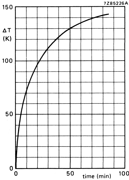
Fig. 4 Temperature increase versus operation time.
