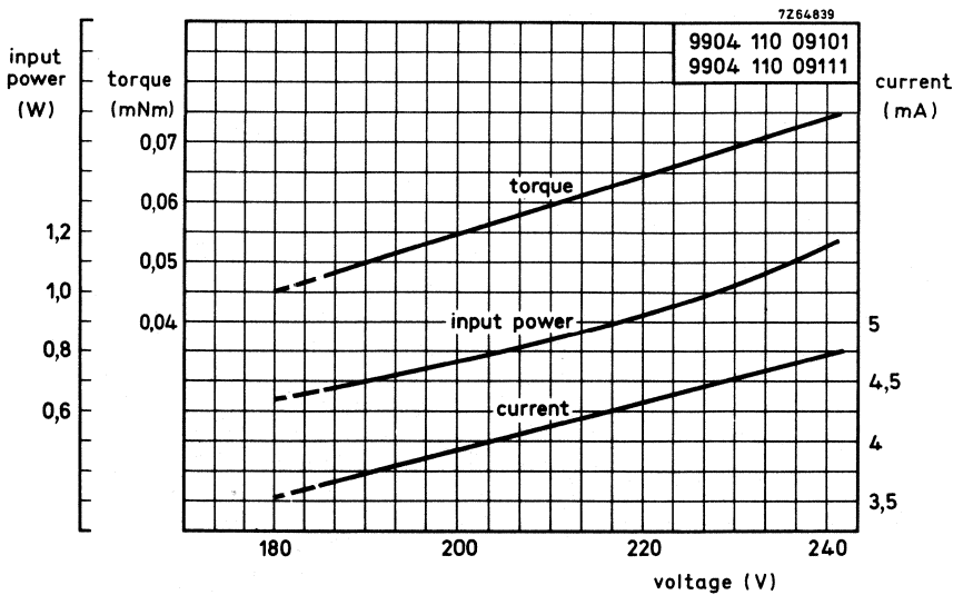
Fig. 4d Typical curves of motors used with a series resistor of 47 kΩ.
