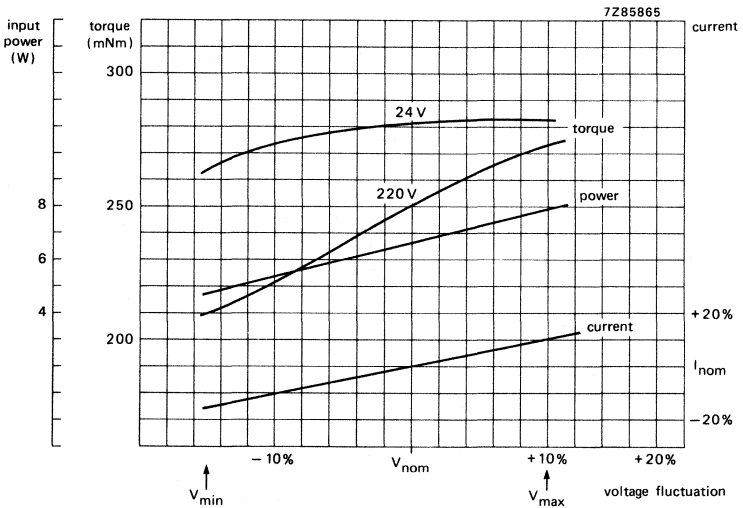
Fig. 4 Typical curves for 60 Hz operation.
