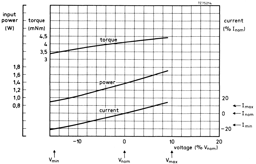
Fig. 2 Typical curves.
