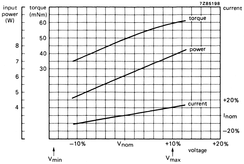
Fig. 3 Typical curves.
