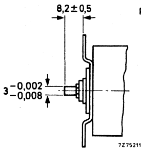
Fig. 1b Version with \phi 3 mm spindle, for combination with gearbox series 9912 200 . . . . .
