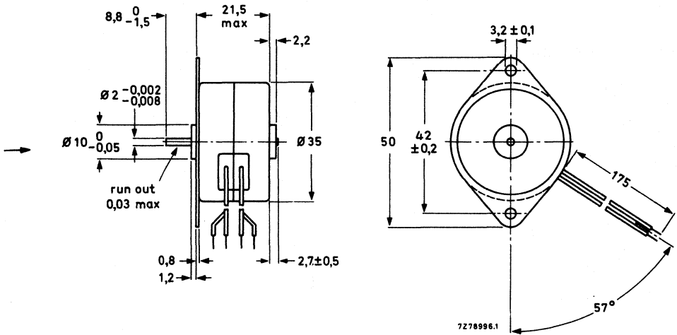
Fig. 1 Version with \varnothing 2 mm spindle. The leads are double insulated (AWG24).
