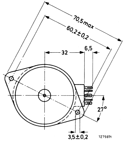
Fig. 1 Version with \phi 1,8 mm spindle.
