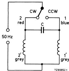
Fig. 2 Connection of the phasing capacitor.
